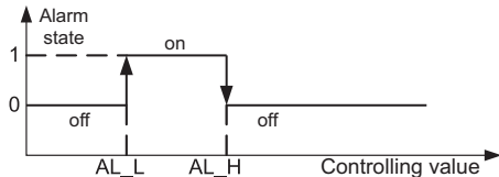
Fig. 21. Alarm types: a) n-on; b) n-off; c) on; d) off.
