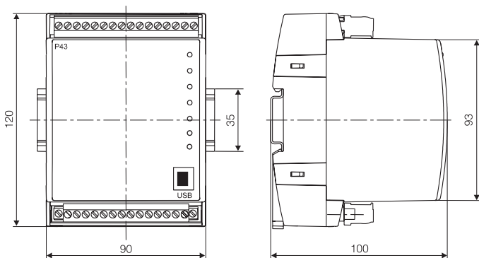
Fig.1 Overall Dimensions and Transducer Fitting Way.
